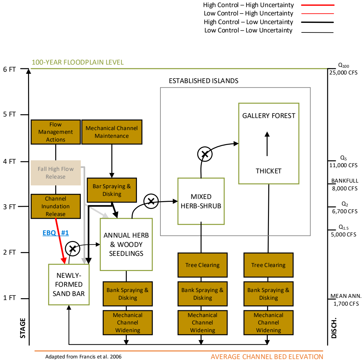
Figure 2. Annual and perennial vegetation establishment sub-model. ⊗ represents the blocking of progression from one successional stage to another through the use of the indicated management action. Actions at bottom right take the channel back to stage-zero riverbed, bare sand similar to newly formed sand bars. Dark colored boxes that stand out represent areas of high focus during the Extension. Light colored boxes that fade into the background represent areas of low focus during the Extension. Model adapted from Francis et al. 2006.
