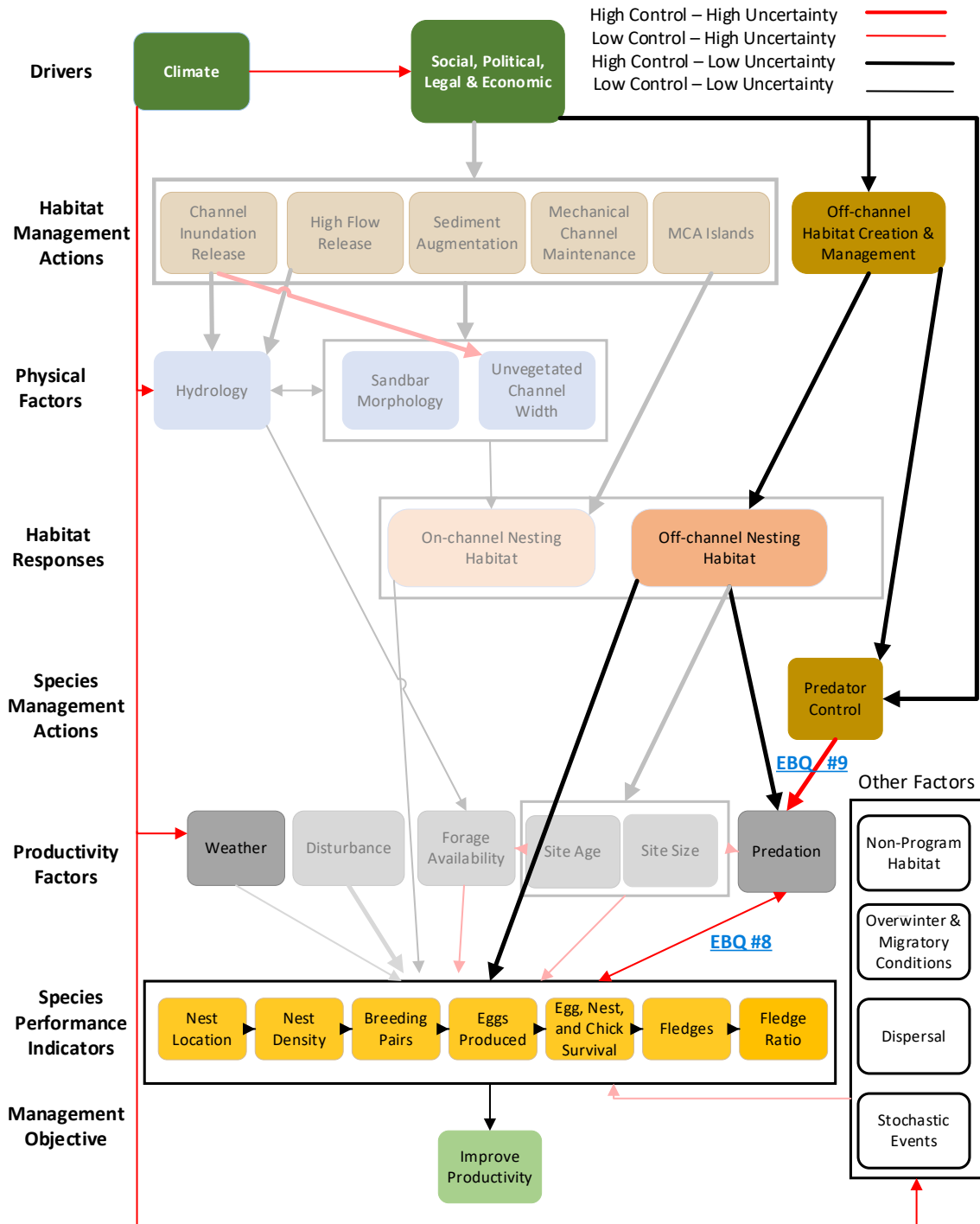
Figure 5. Plover and Tern Conceptual Ecological Model (CEM). Dark colored boxes that stand out represent areas of high focus during the Extension. Light colored boxes that fade into the background represent areas of low focus during the Extension.
