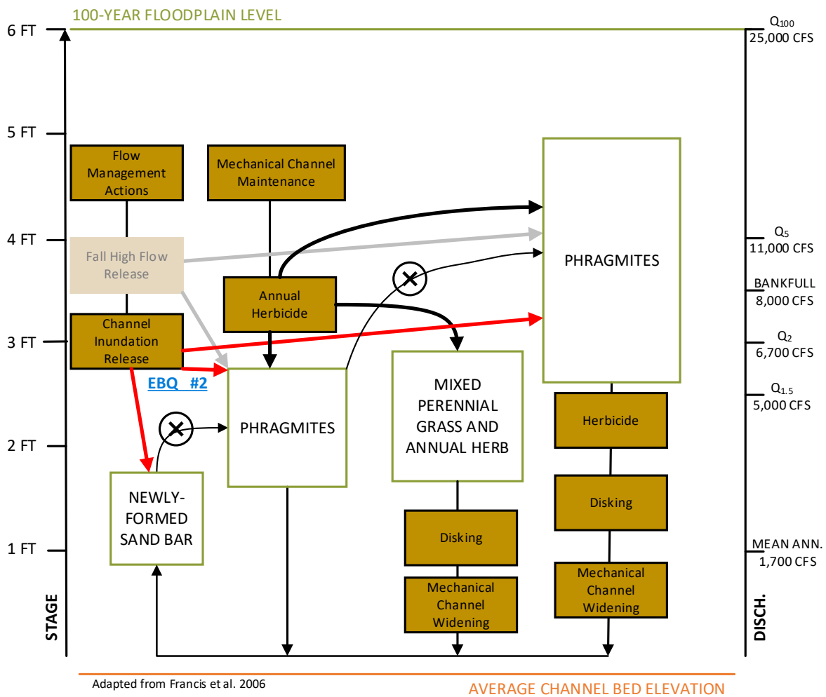
Figure 3. Phragmites sub-model. ⊗ represents the blocking of progression from one successional stage to another through the use of the indicated management action. Actions at bottom right take the channel back to stage-zero riverbed, bare sand similar to newly formed sand bars. Dark colored boxes that stand out represent areas of high focus during the Extension. Light colored boxes that fade into the background represent areas of low focus during the Extension. Model adapted from Francis et al. 2006 .
