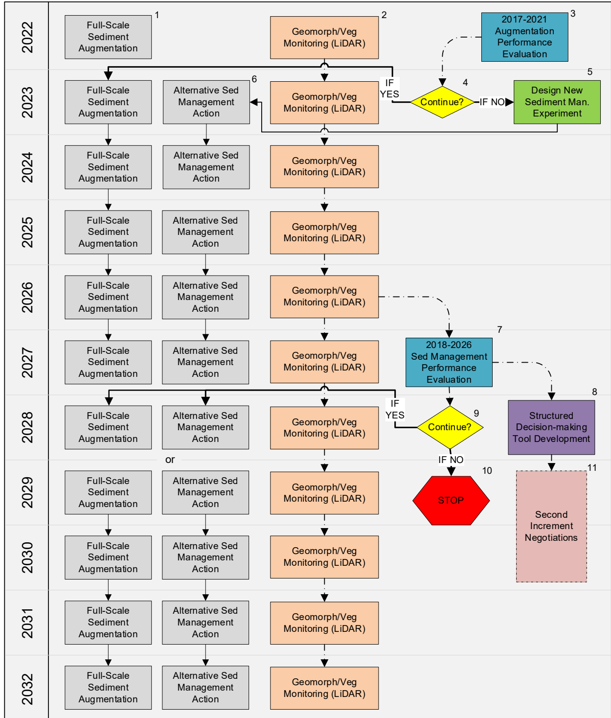
Figure 6. Sediment Augmentation Activity Diagram
