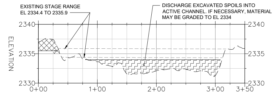
PILOT CHANNEL - PROFILE H: 1 IN = 100 FT, V: 1 IN = 10 FT
