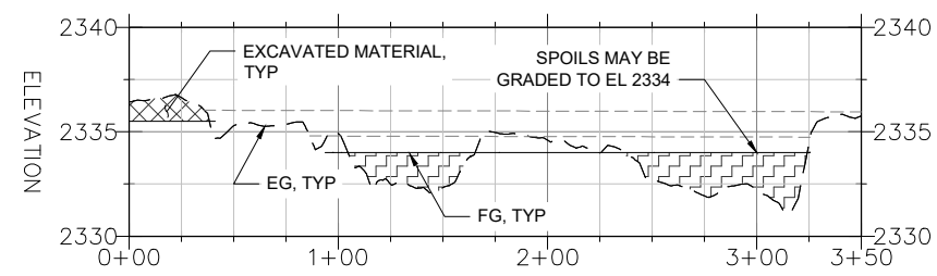
PILOT CHANNEL - PROFILE H: 1 IN = 100 FT, V: 1 IN = 10 FT
