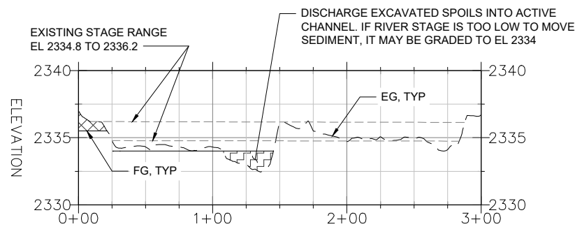
PILOT CHANNEL - PROFILE H: 1 IN = 100 FT, V: 1 IN = 10 FT
